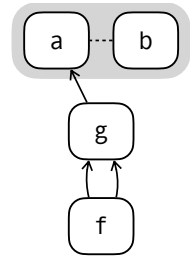
Fig. 2. An example e-graph.
